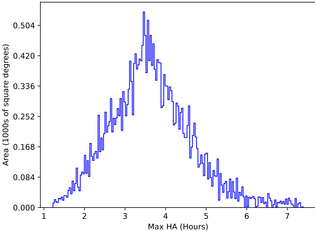
start_date_do-270v3.4_10yrs All sky g band: Max HA
