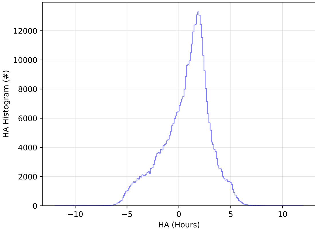
start_date_do-270v3.4_10yrs WFD z band: HA Histogram
