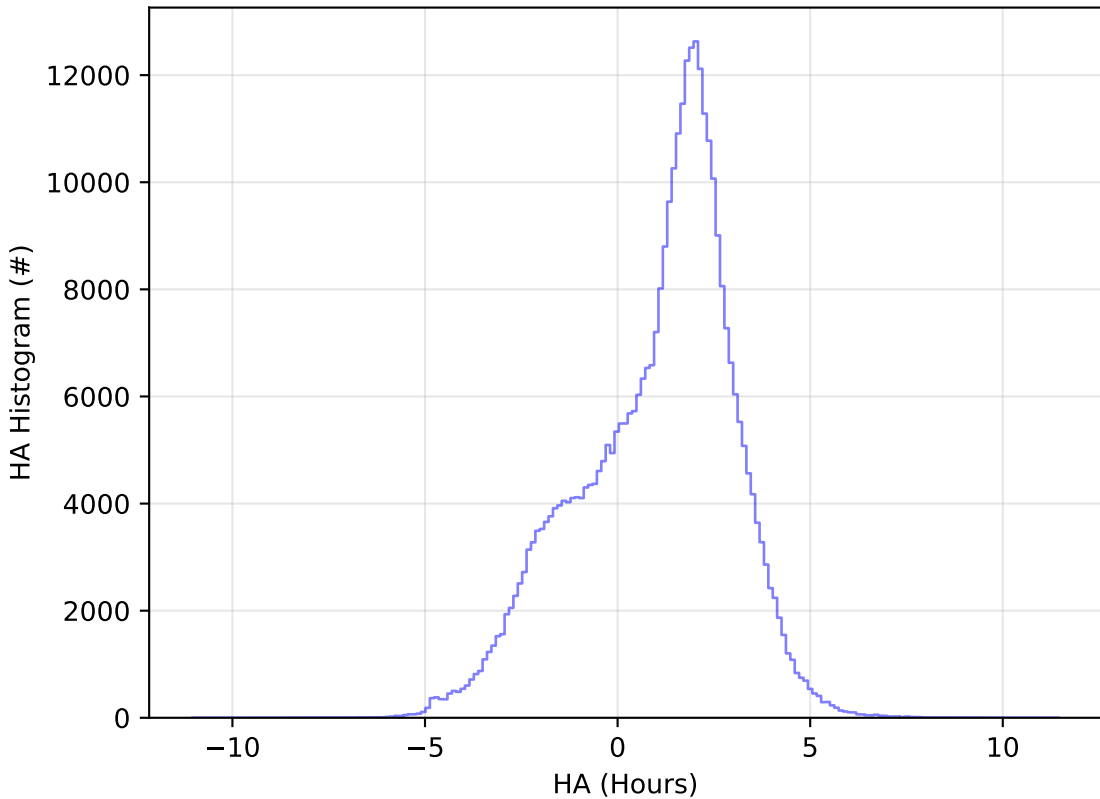
start_date_do-270v3.4_10yrs WFD y band: HA Histogram
