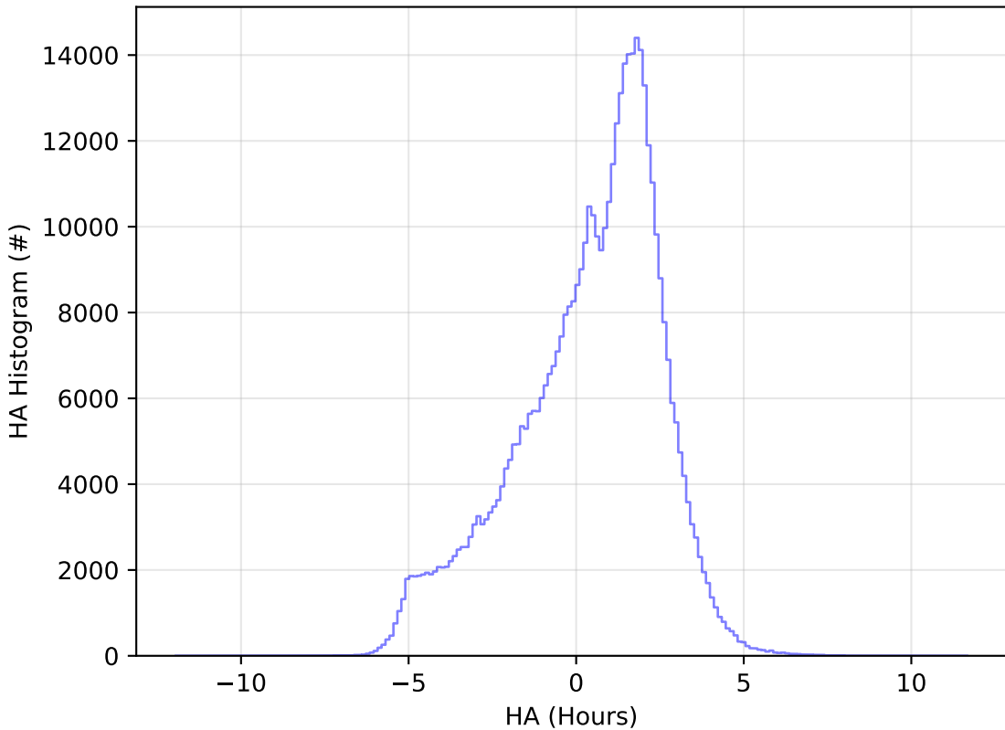
start_date_do-270v3.4_10yrs WFD r band: HA Histogram
