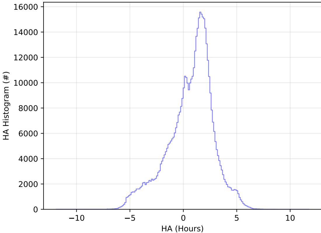
start_date_do-270v3.4_10yrs WFD i band: HA Histogram
