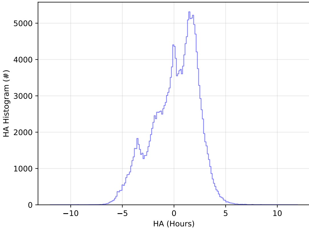
start_date_do-270v3.4_10yrs WFD g band: HA Histogram
