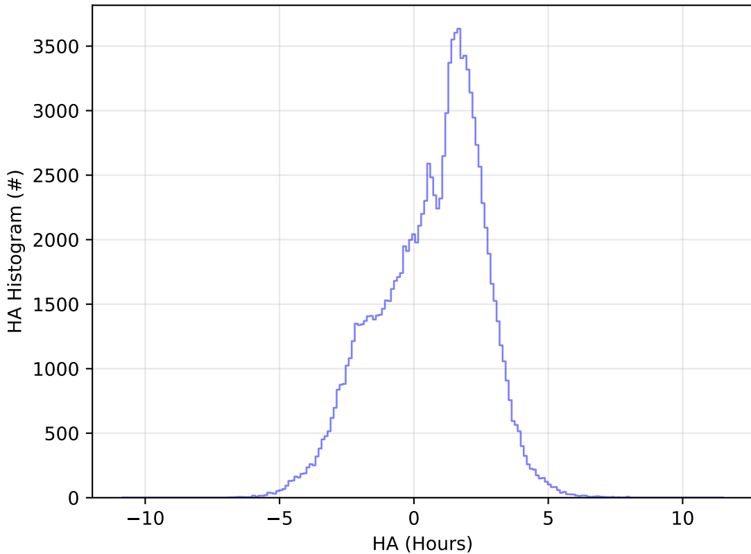
start_date_do-270v3.4_10yrs All sky u band: HA Histogram
