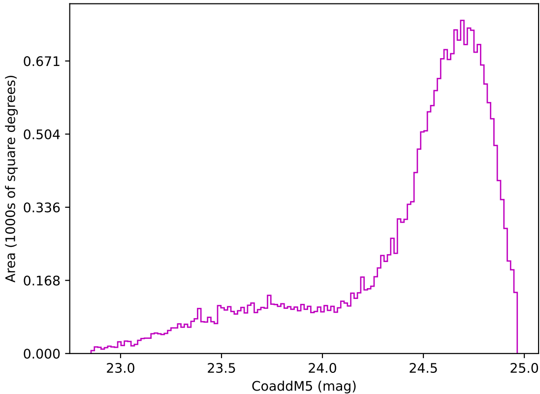
start_date_do-270v3.4_10yrs Yr 1 z band: CoaddM5
