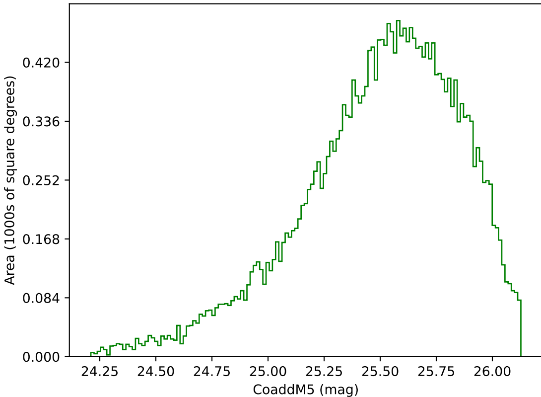
start_date_do-270v3.4_10yrs Yr 1 g band: CoaddM5
