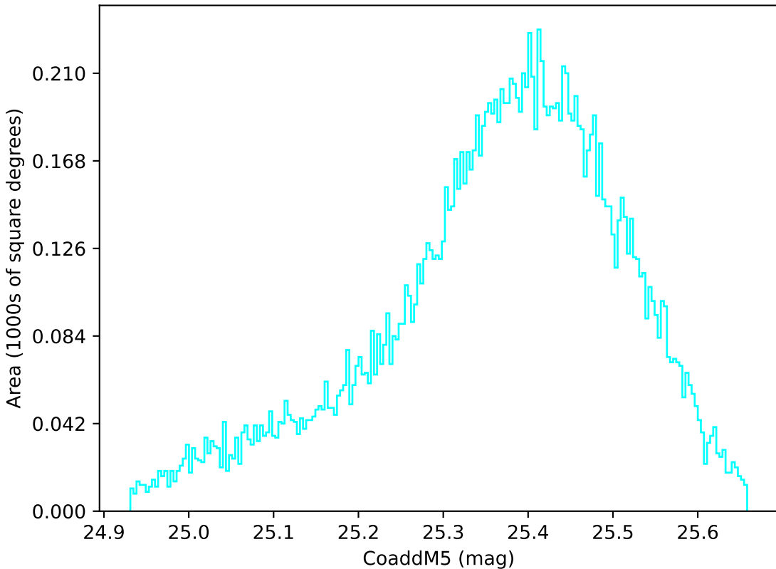
start_date_do-270v3.4_10yrs WFD u band: CoaddM5
