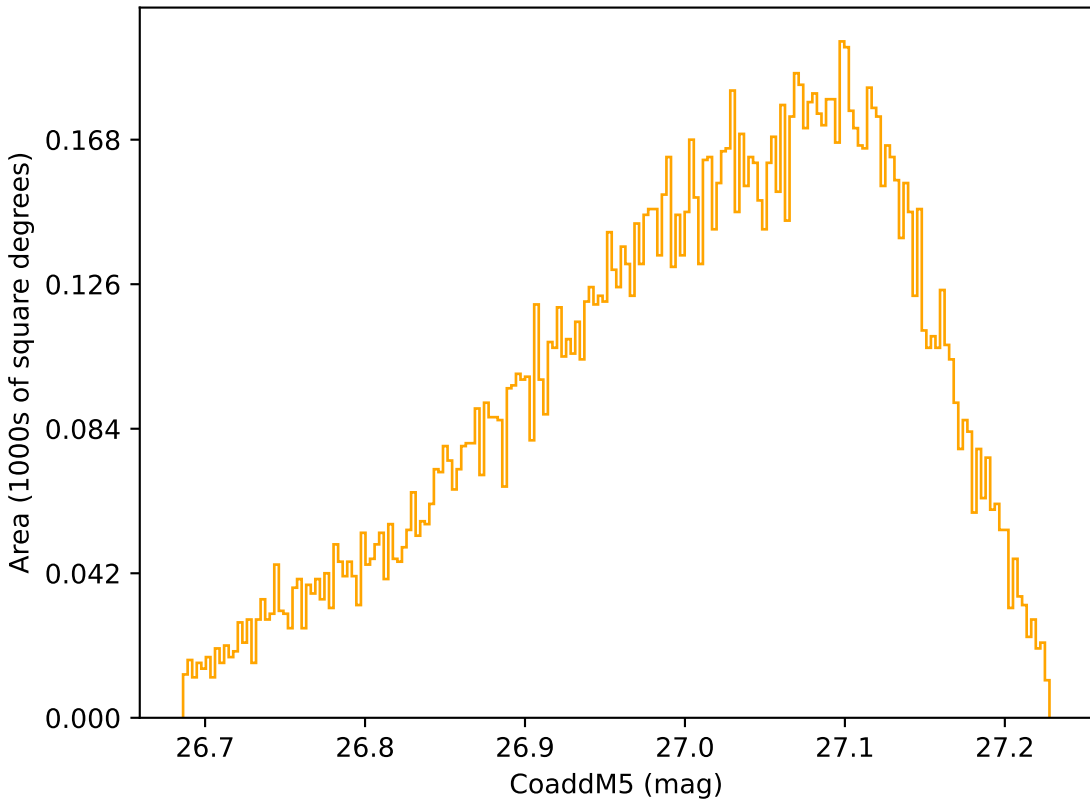
start_date_do-270v3.4_10yrs WFD r band: CoaddM5
