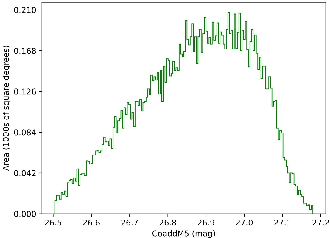
start_date_do-270v3.4_10yrs WFD g band: CoaddM5
