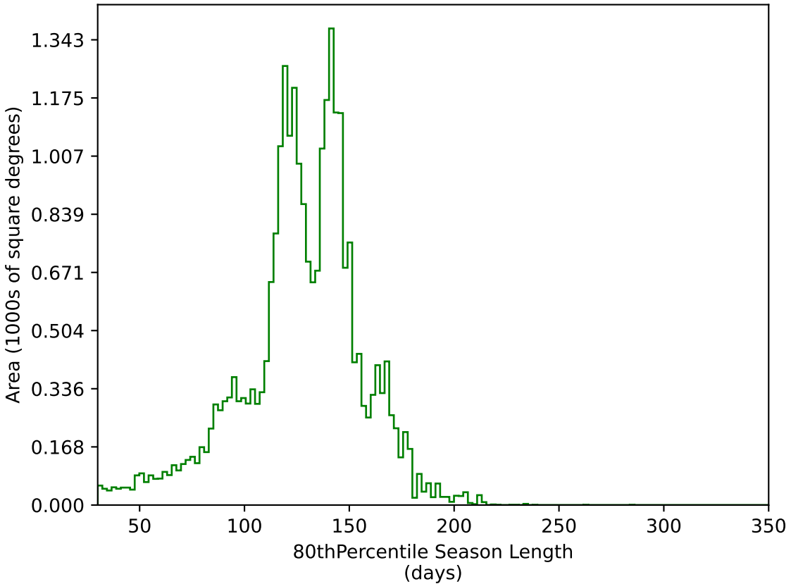
start_date_do-270v3.4_10yrs All sky g band: 80thPercentile Season Length
