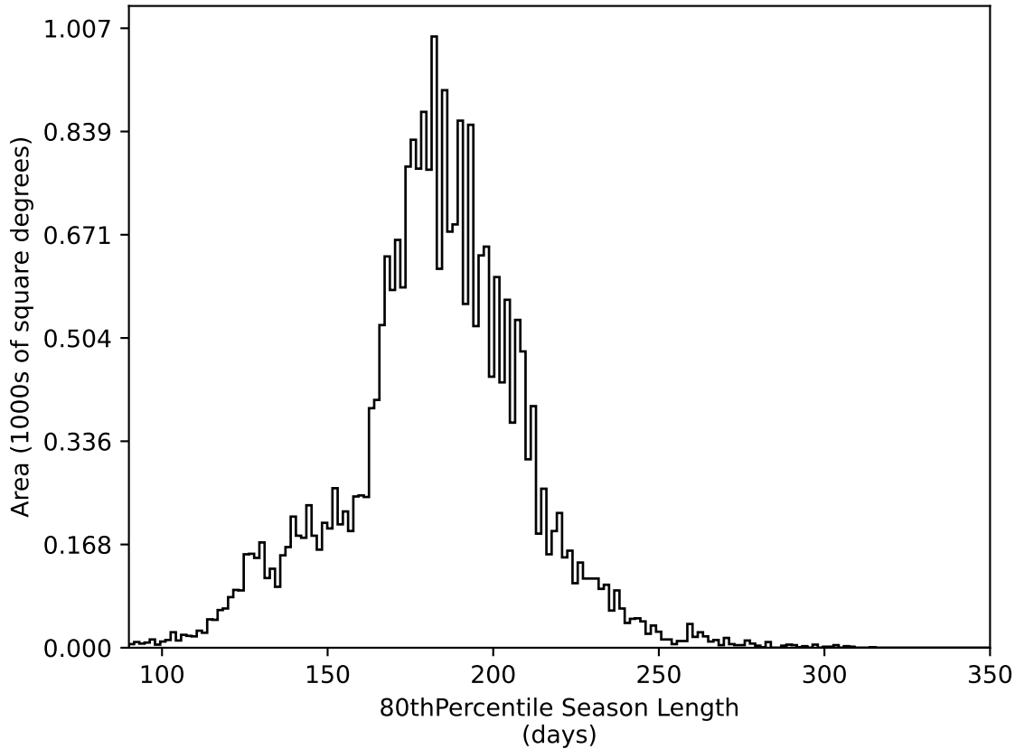
start_date_do-270v3.4_10yrs All sky all bands: 80thPercentile Season Length
