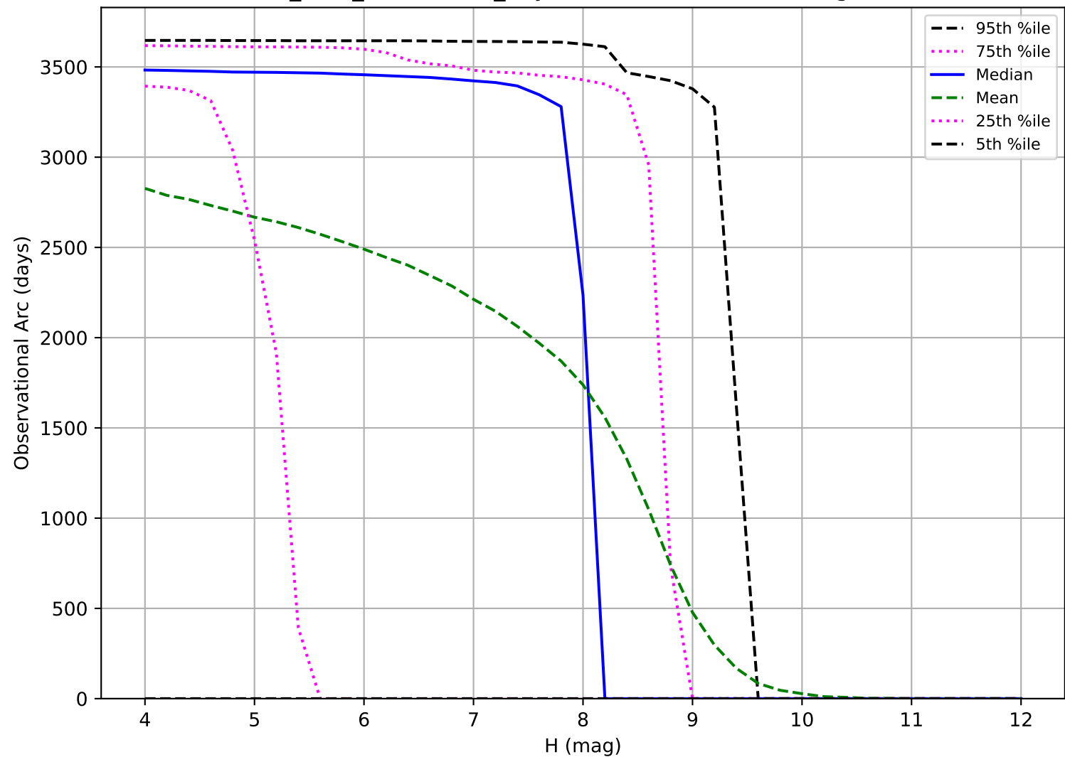
start_date_do-180v3.4_10yrs: Observational Arc Length TNO
