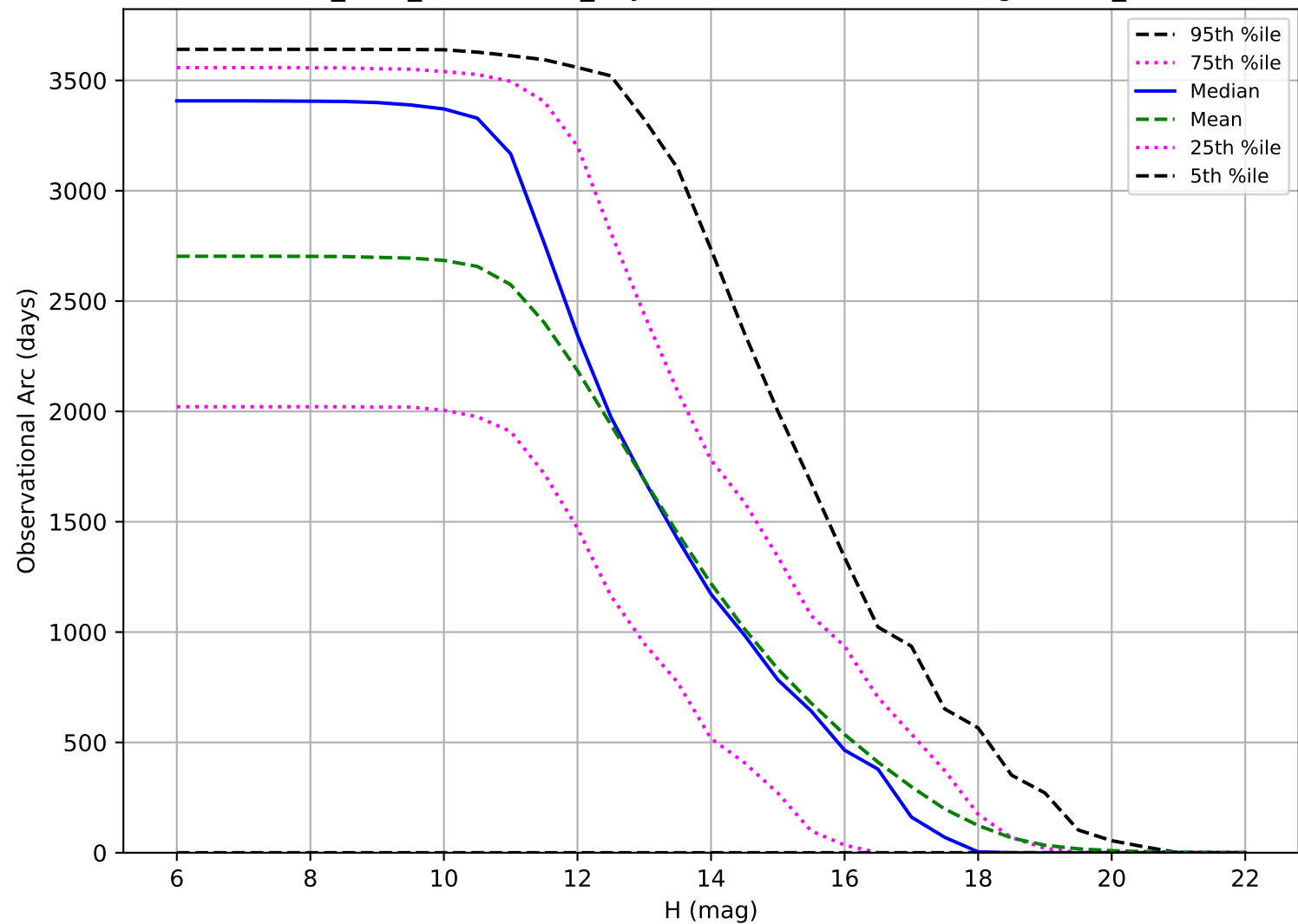
start_date_do-180v3.4_10yrs: Observational Arc Length OCC_r5
