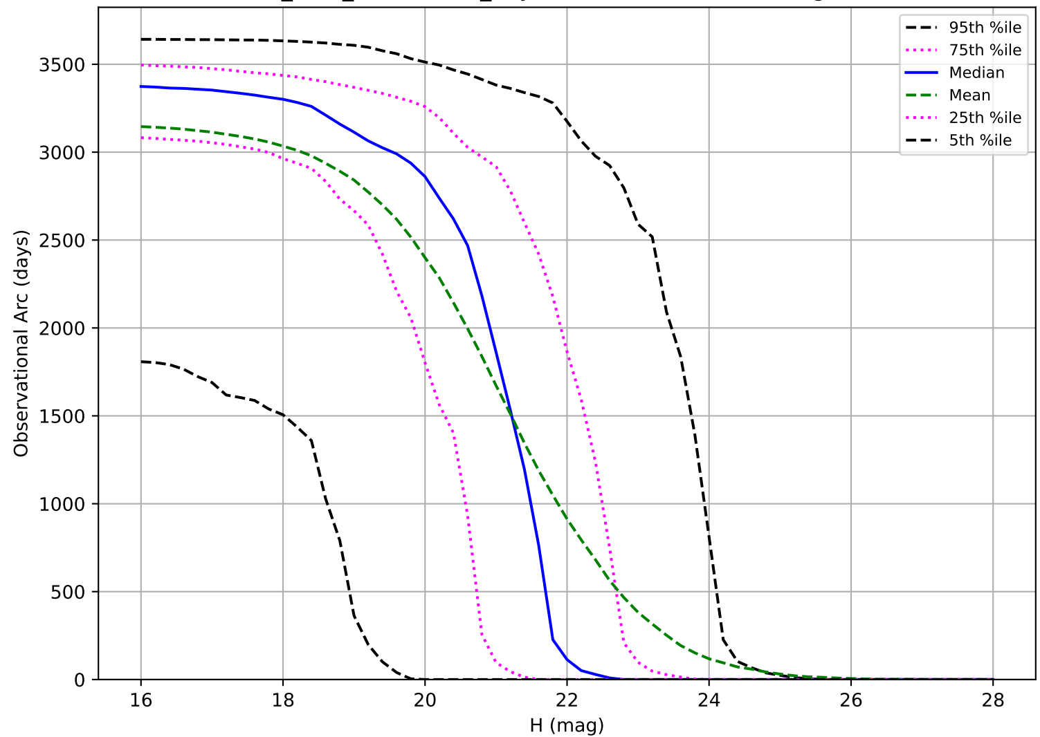
start_date_do-180v3.4_10yrs: Observational Arc Length NEO
