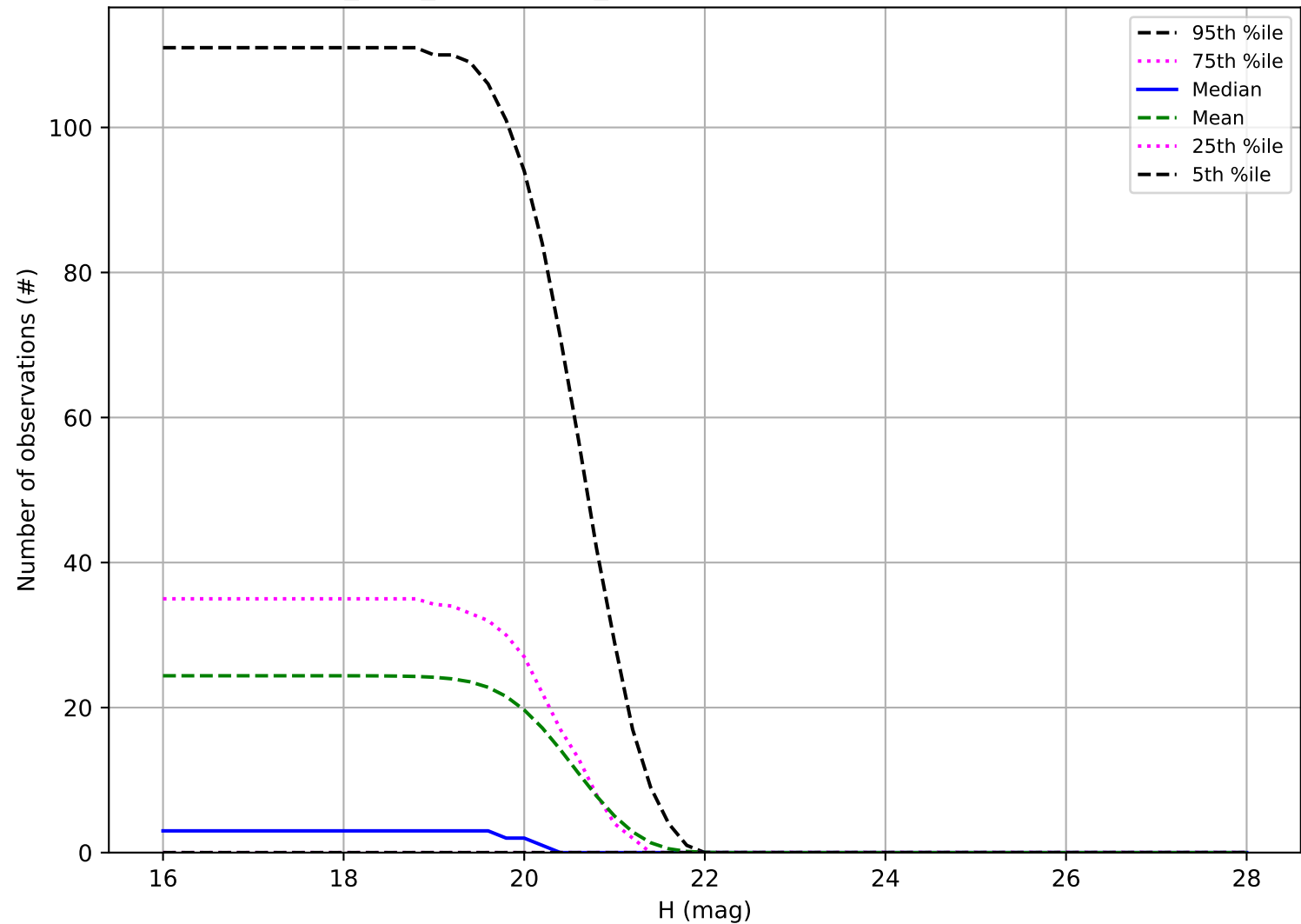
start_date_do-180v3.4_10yrs: Number of observations Vatira
