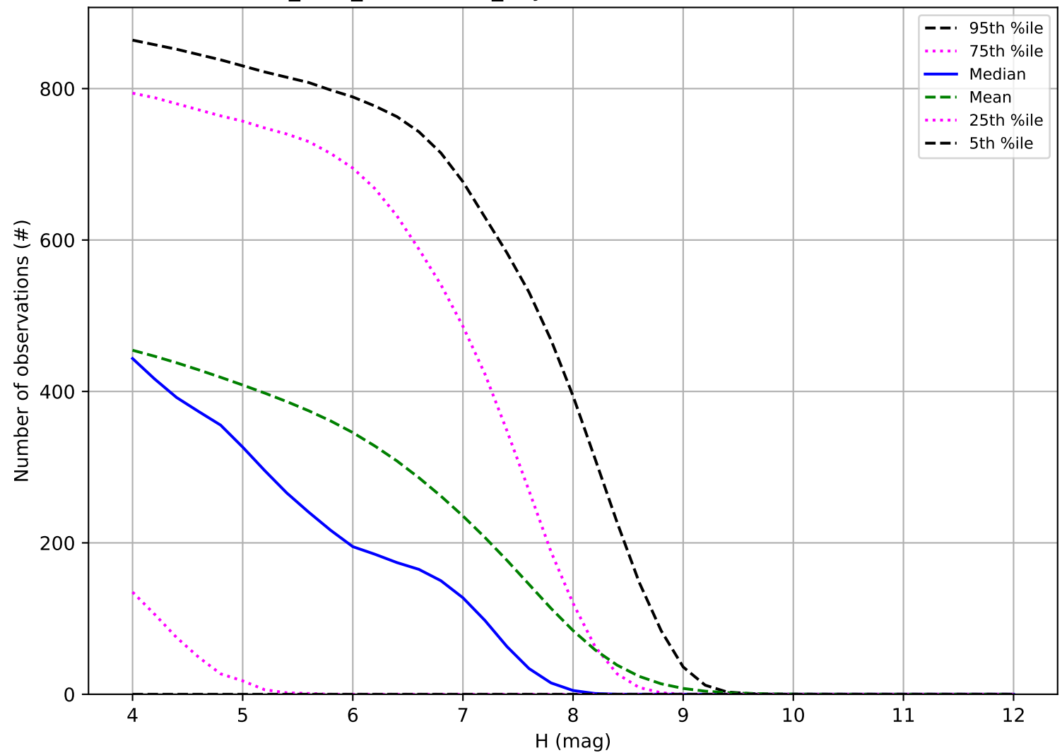
start_date_do-180v3.4_10yrs: Number of observations TNO
