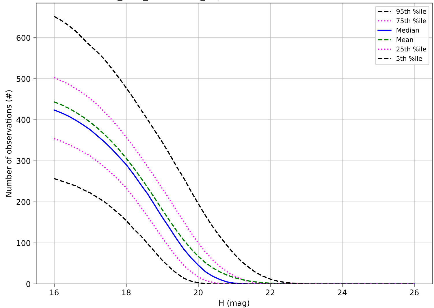
start_date_do-180v3.4_10yrs: Number of observations MBA
