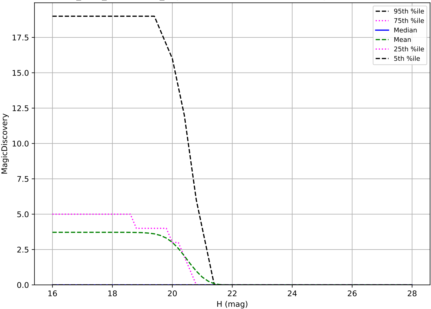
start_date_do-180v3.4_10yrs: Vatira 6 detections in 60 nights detection loss
