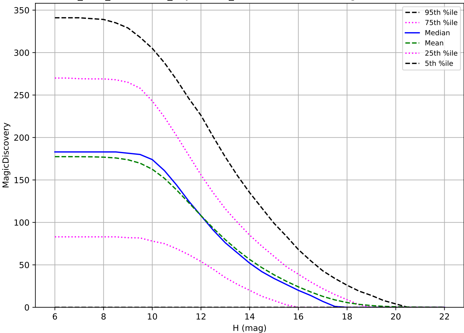
start_date_do-180v3.4_10yrs: OCC_r5 6 detections in 60 nights detection loss
