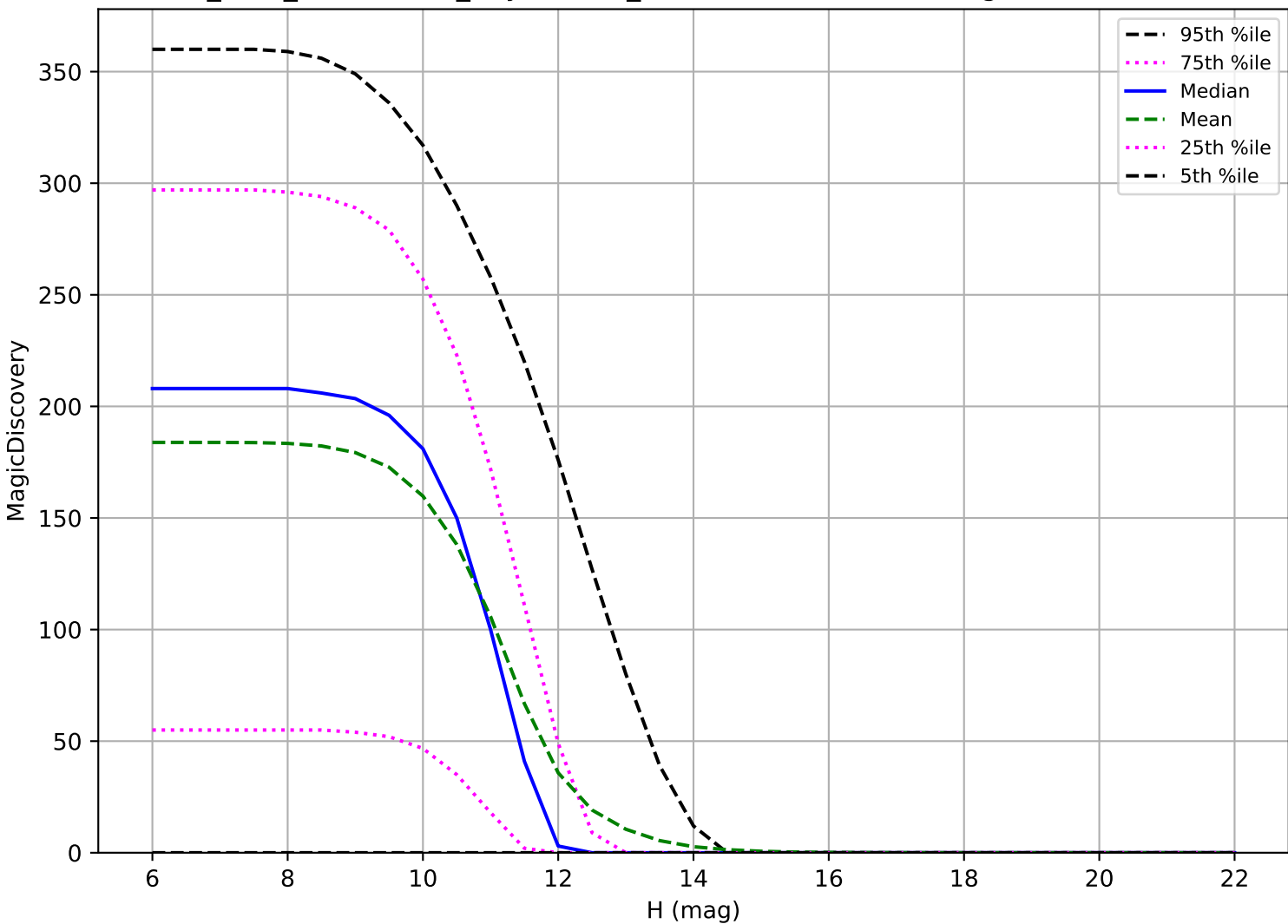
start_date_do-180v3.4_10yrs: OCC_r20 6 detections in 60 nights detection loss
