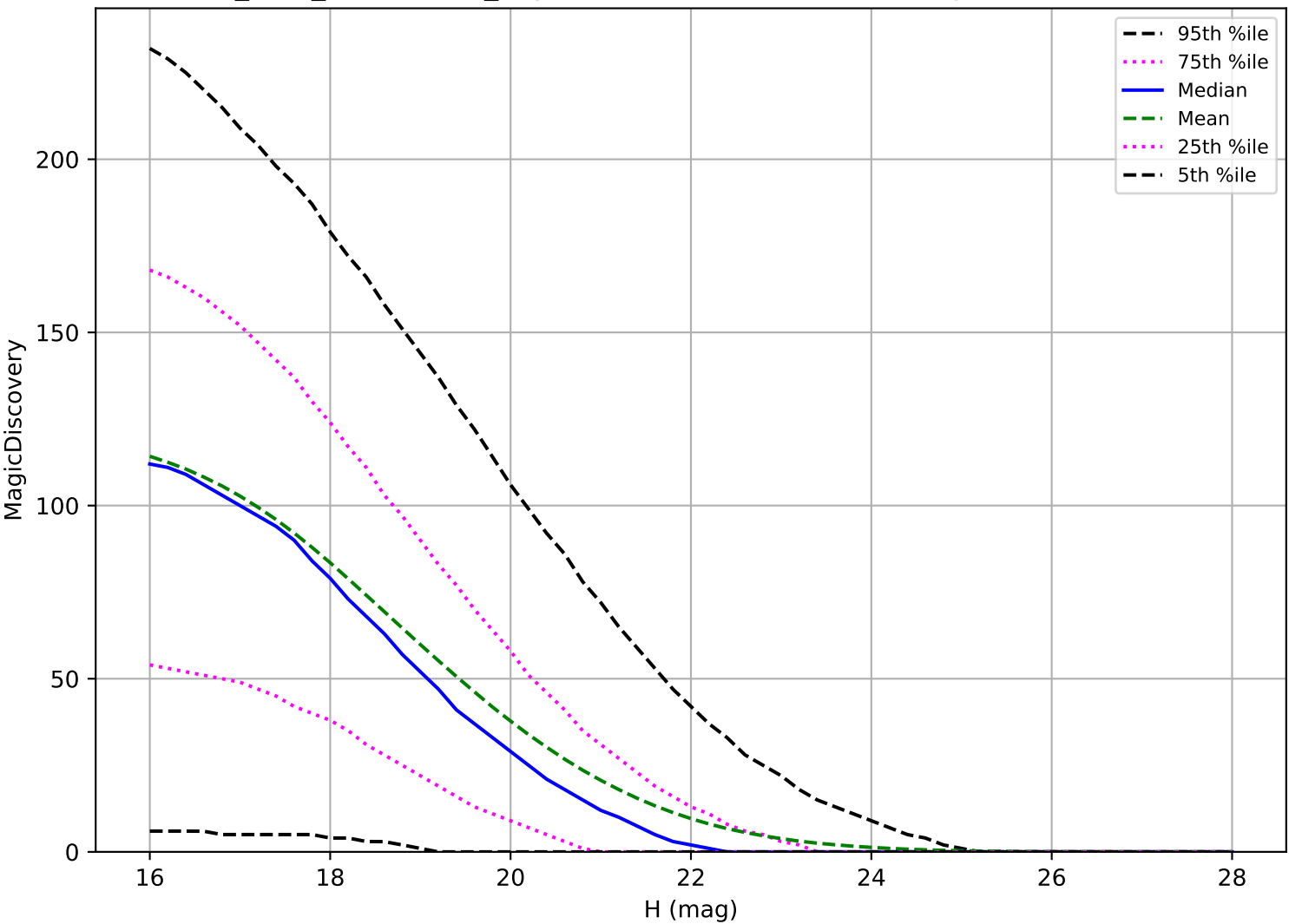
start_date_do-180v3.4_10yrs: NEO 6 detections in 60 nights detection loss
