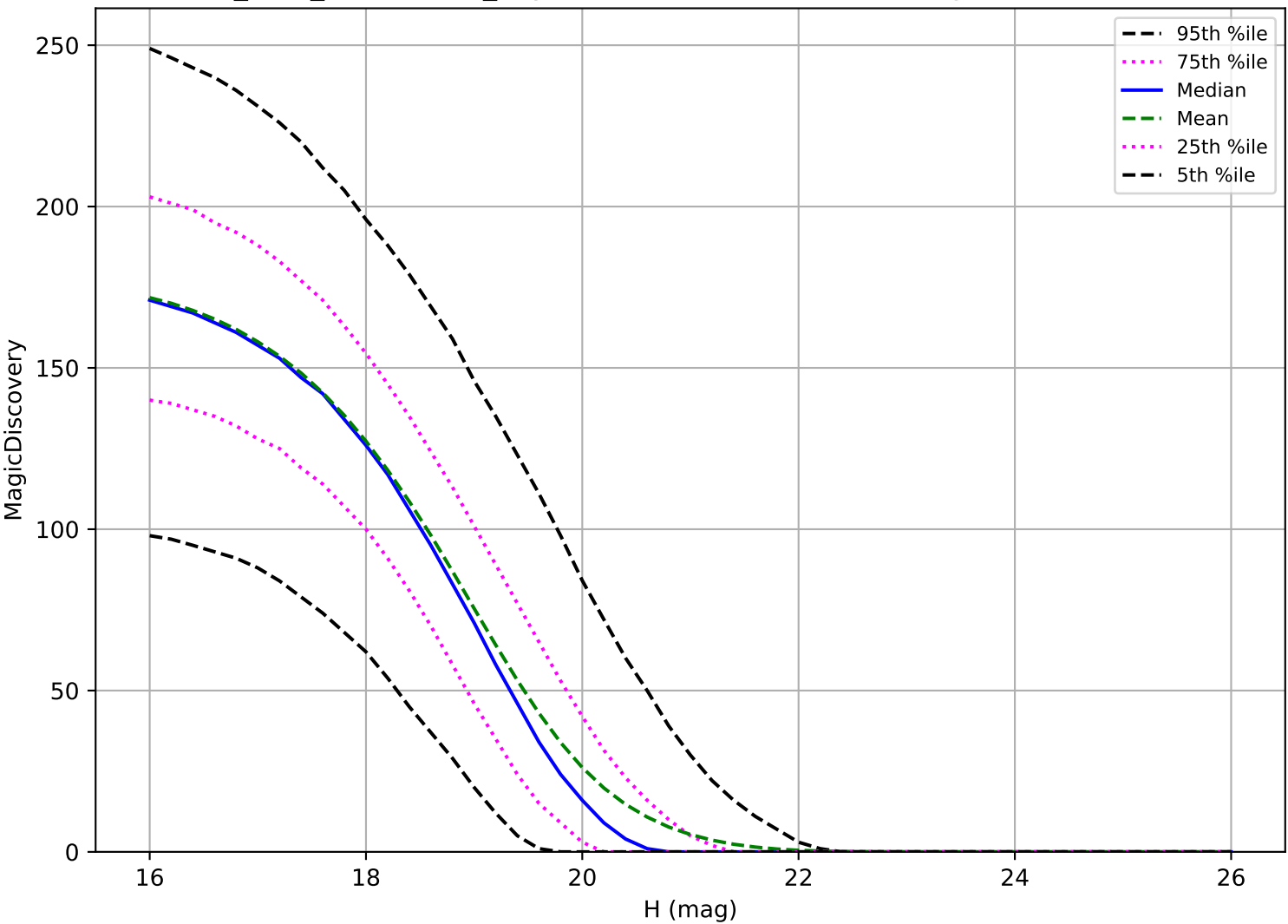
start_date_do-180v3.4_10yrs: MBA 6 detections in 60 nights detection loss
