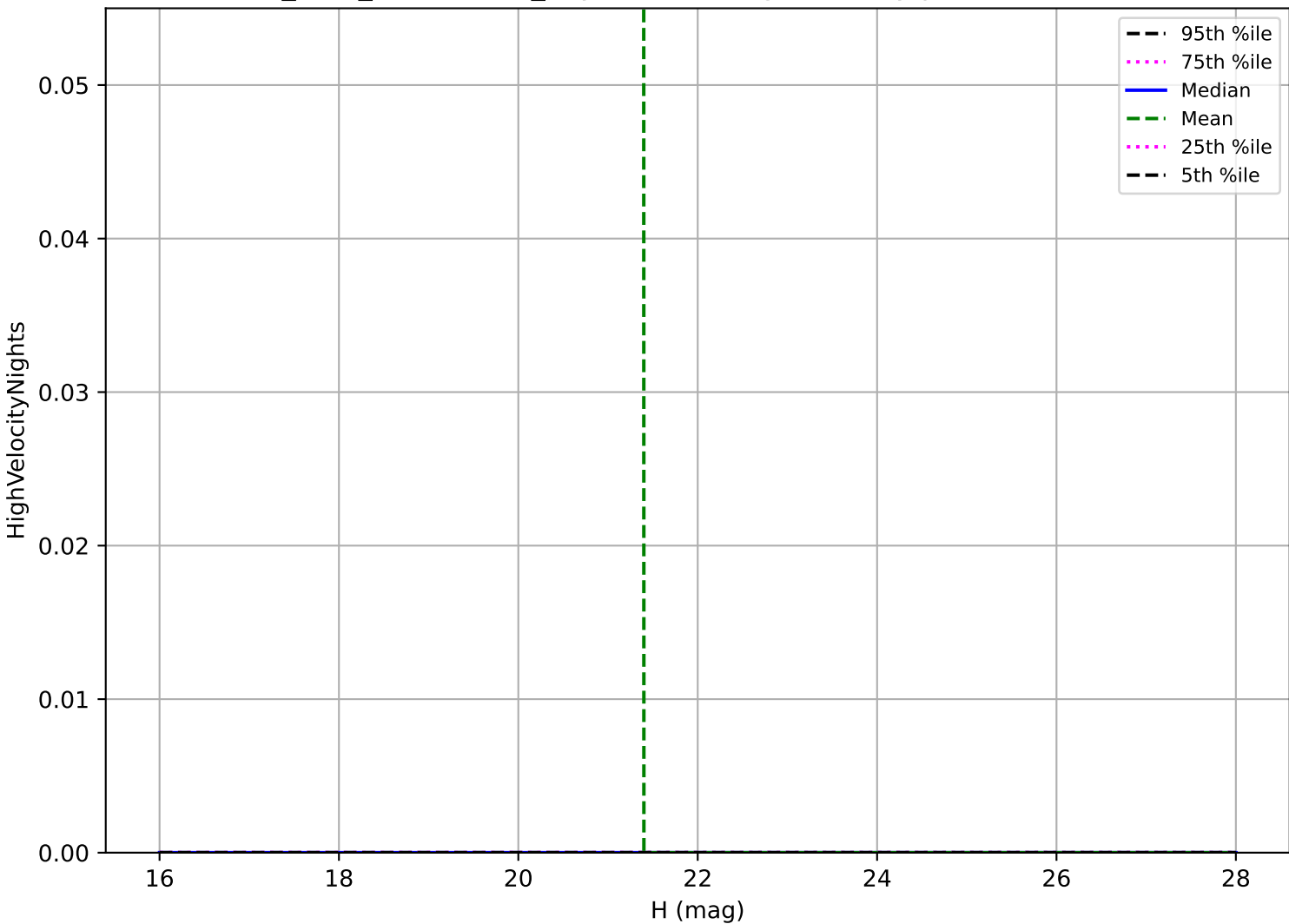
start_date_do-180v3.4_10yrs: Vatira High velocity pair detection loss
