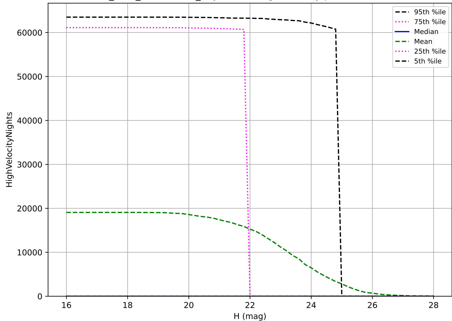
start_date_do-180v3.4_10yrs: NEO High velocity pair detection loss
