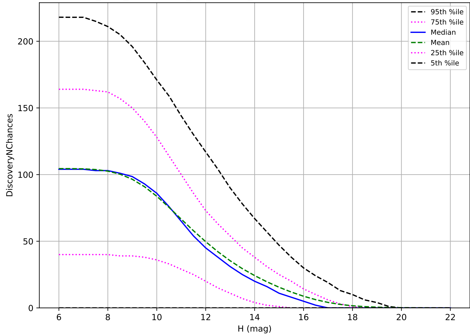
start_date_do-180v3.4_10yrs: OCC_r5 3 pairs in 15 nights detection loss
