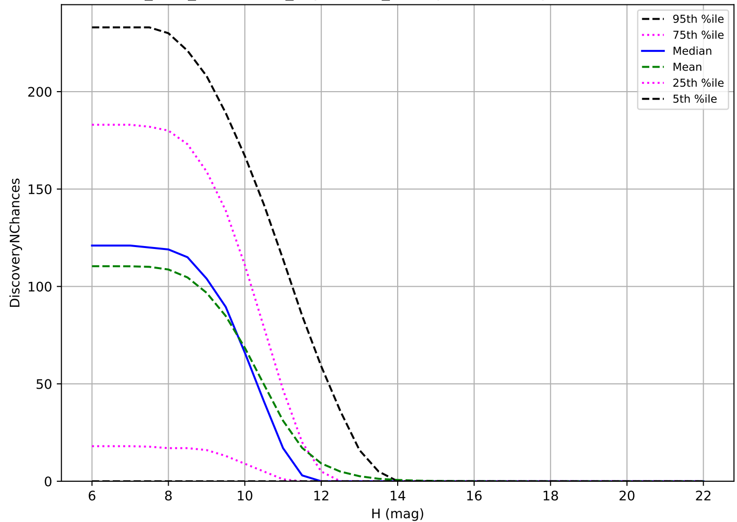
start_date_do-180v3.4_10yrs: OCC_r20 3 pairs in 15 nights detection loss
