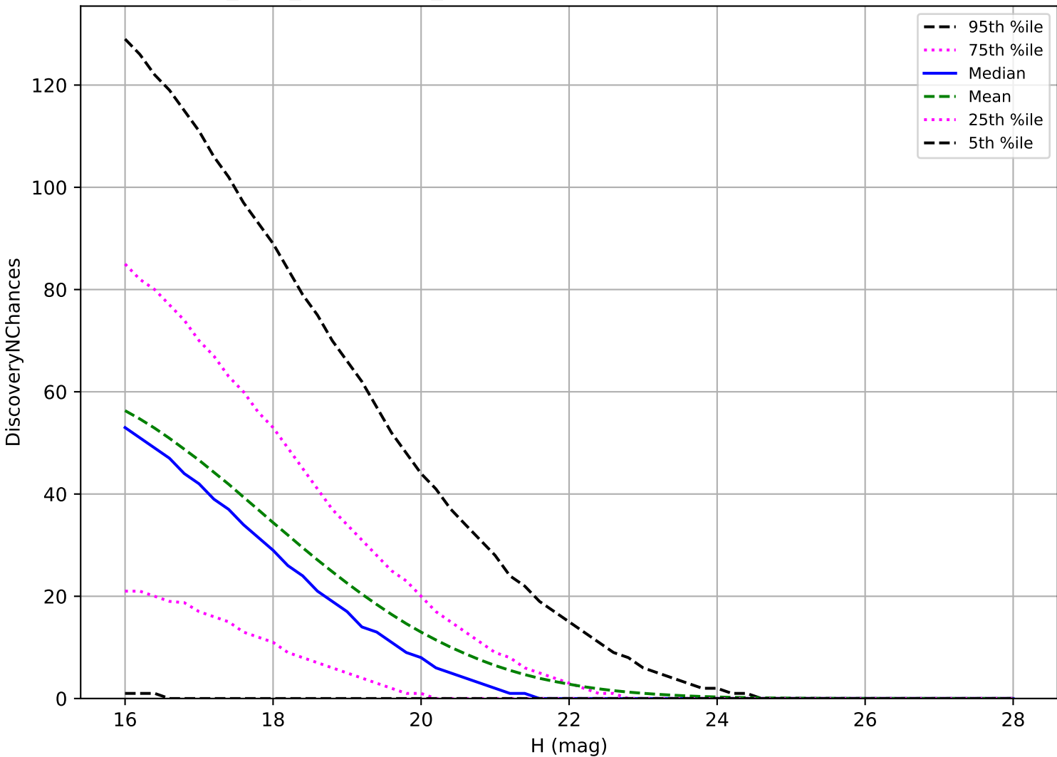
start_date_do-180v3.4_10yrs: NEO 3 pairs in 15 nights detection loss
