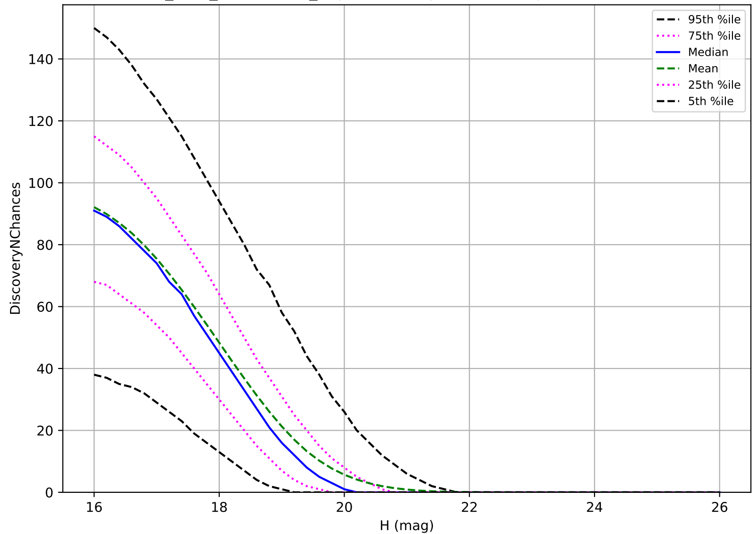
start_date_do-180v3.4_10yrs: MBA 3 pairs in 15 nights detection loss
