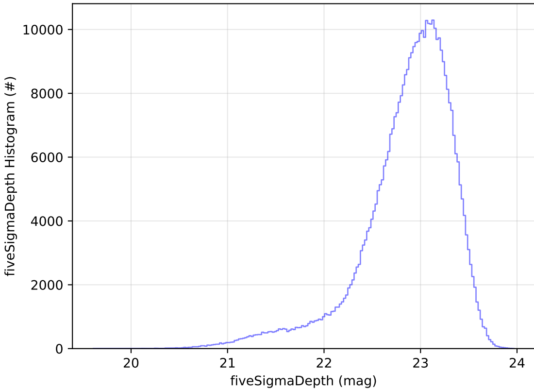
start_date_do-180v3.4_10yrs z: fiveSigmaDepth Histogram
