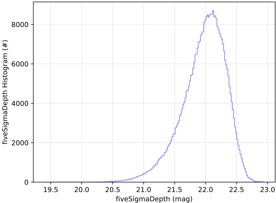
start_date_do-180v3.4_10yrs y: fiveSigmaDepth Histogram
