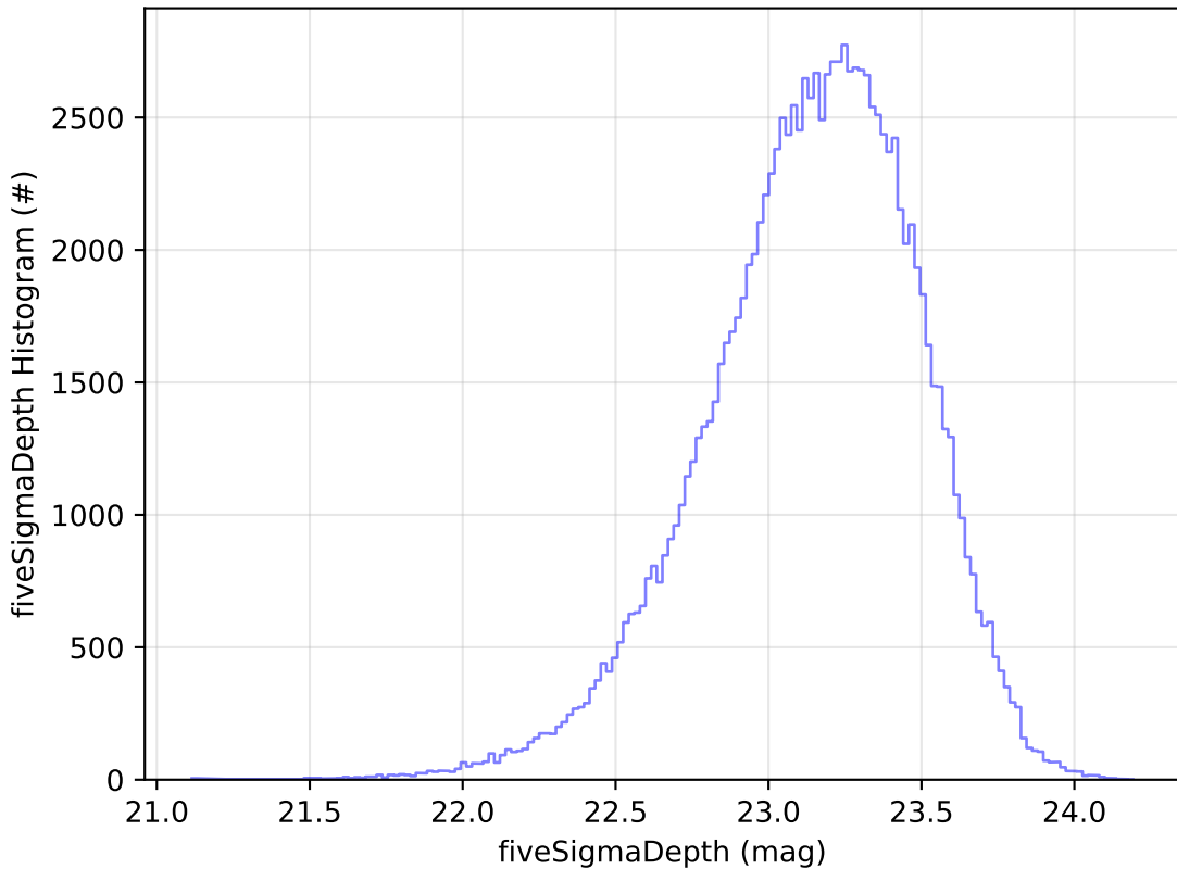
start_date_do-180v3.4_10yrs u: fiveSigmaDepth Histogram
