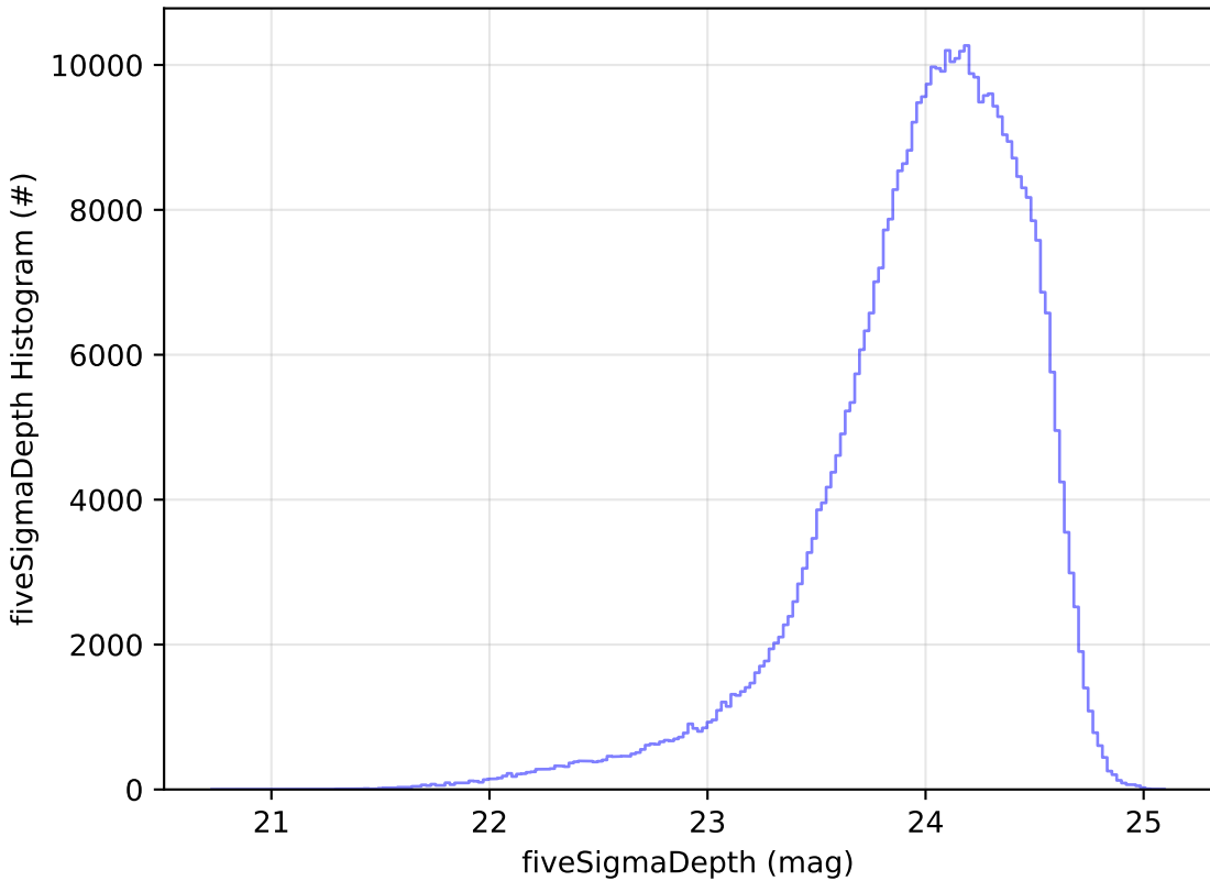
start_date_do-180v3.4_10yrs r: fiveSigmaDepth Histogram
