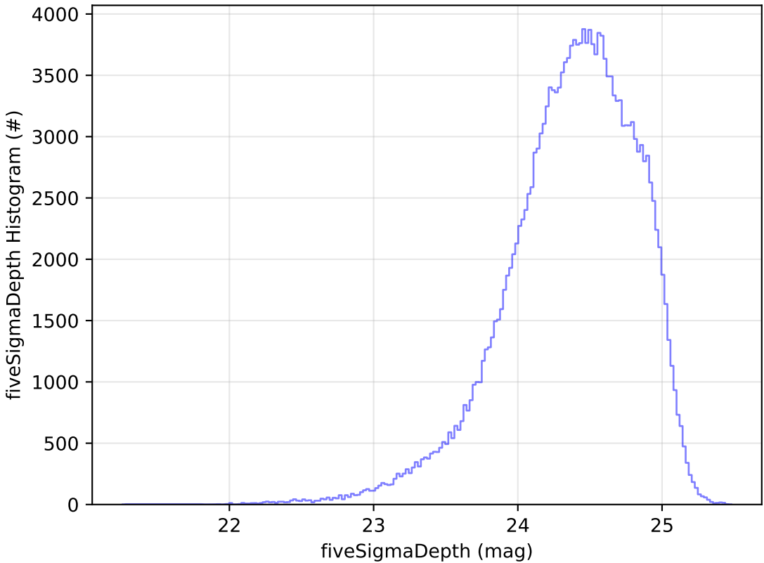
start_date_do-180v3.4_10yrs g: fiveSigmaDepth Histogram
