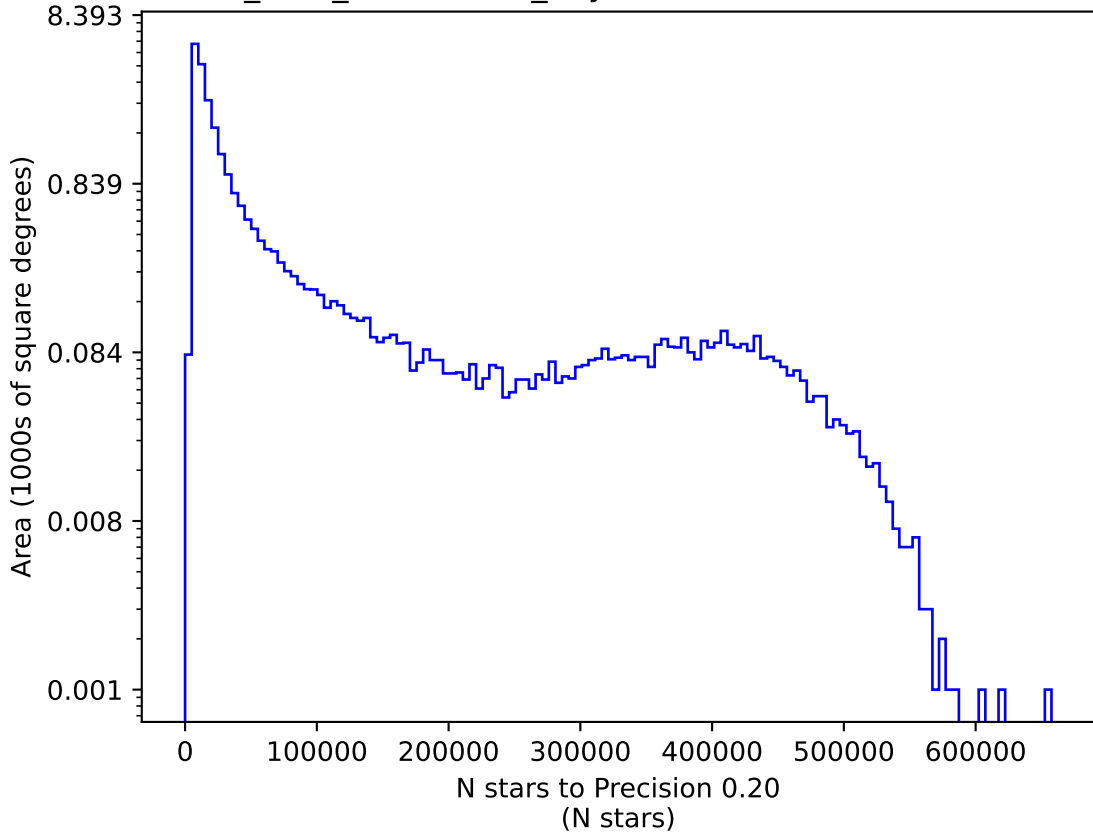
start_date_do-180v3.4_10yrs i: N stars to Precision 0.20
