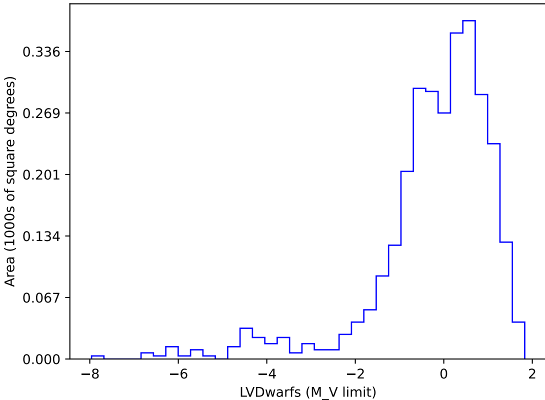
start_date_do-180v3.4_10yrs gi SCP: LVDwarfs
