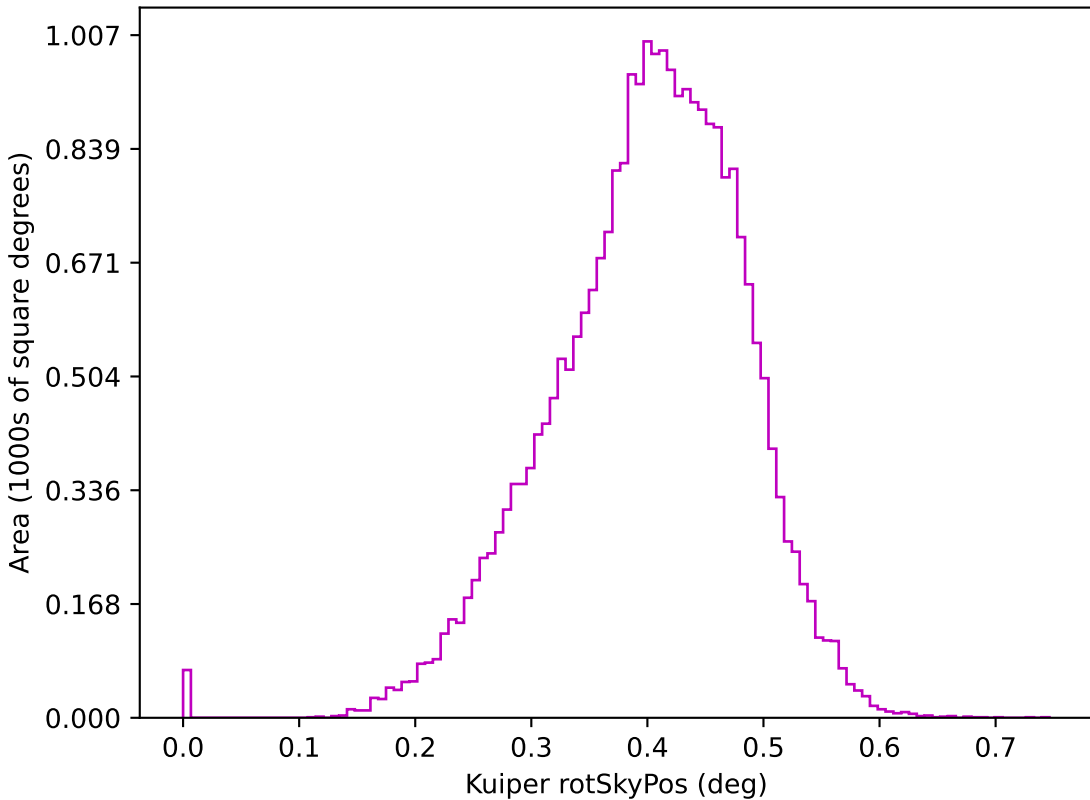
start_date_do-180v3.4_10yrs z: Kuiper rotSkyPos
