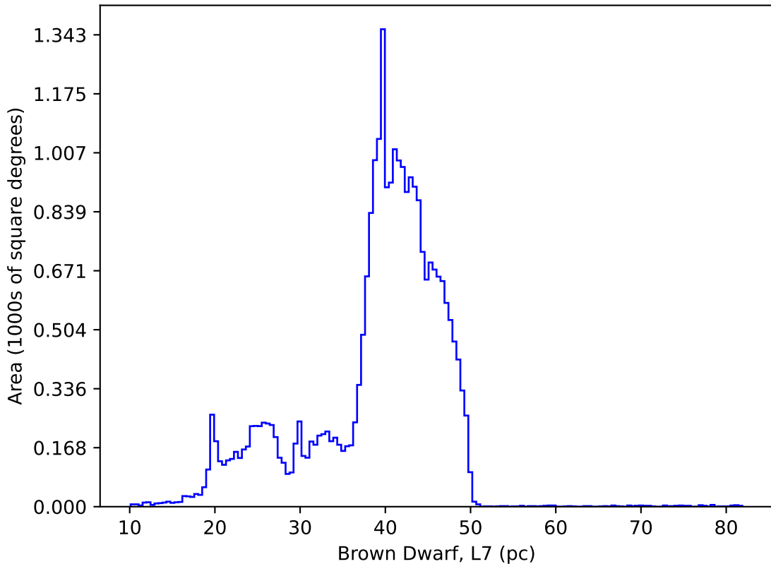
start_date_do-180v3.4_10yrs : Brown Dwarf, L7
