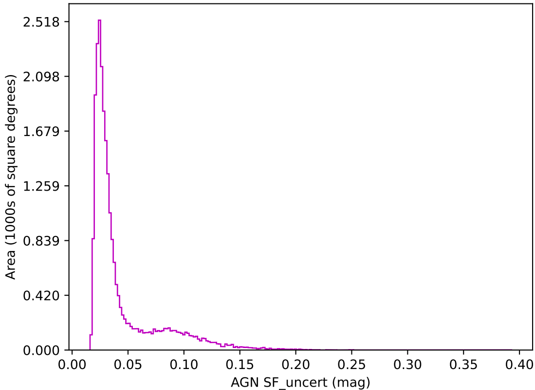
start_date_do-180v3.4_10yrs z band: AGN SF_uncert
