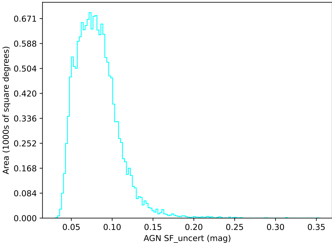
start_date_do-180v3.4_10yrs u band: AGN SF_uncert
