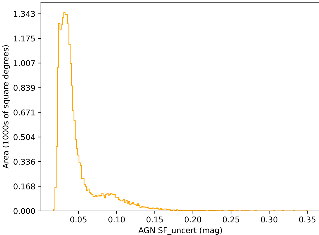
start_date_do-180v3.4_10yrs r band: AGN SF_uncert
