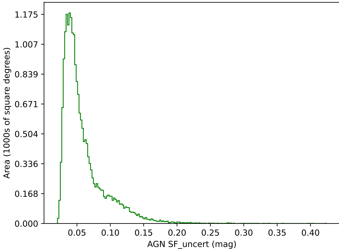
start_date_do-180v3.4_10yrs g band: AGN SF_uncert
