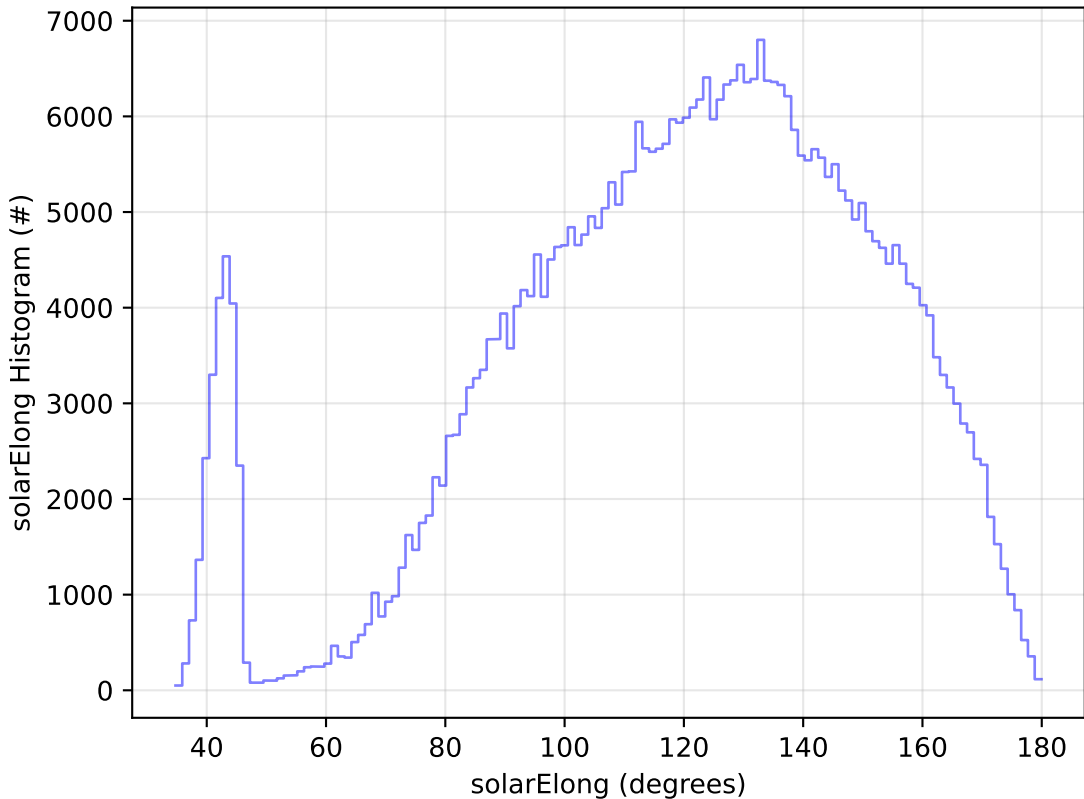
start_date_do-180v3.4_10yrs WFD z band: solarElong Histogram
