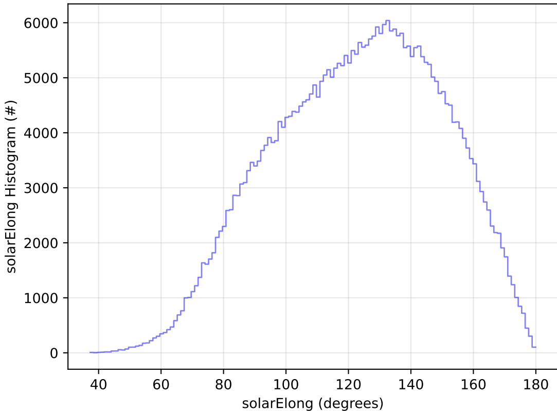
start_date_do-180v3.4_10yrs WFD y band: solarElong Histogram
