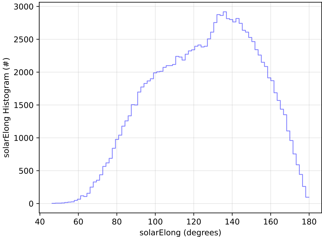
start_date_do-180v3.4_10yrs WFD u band: solarElong Histogram
