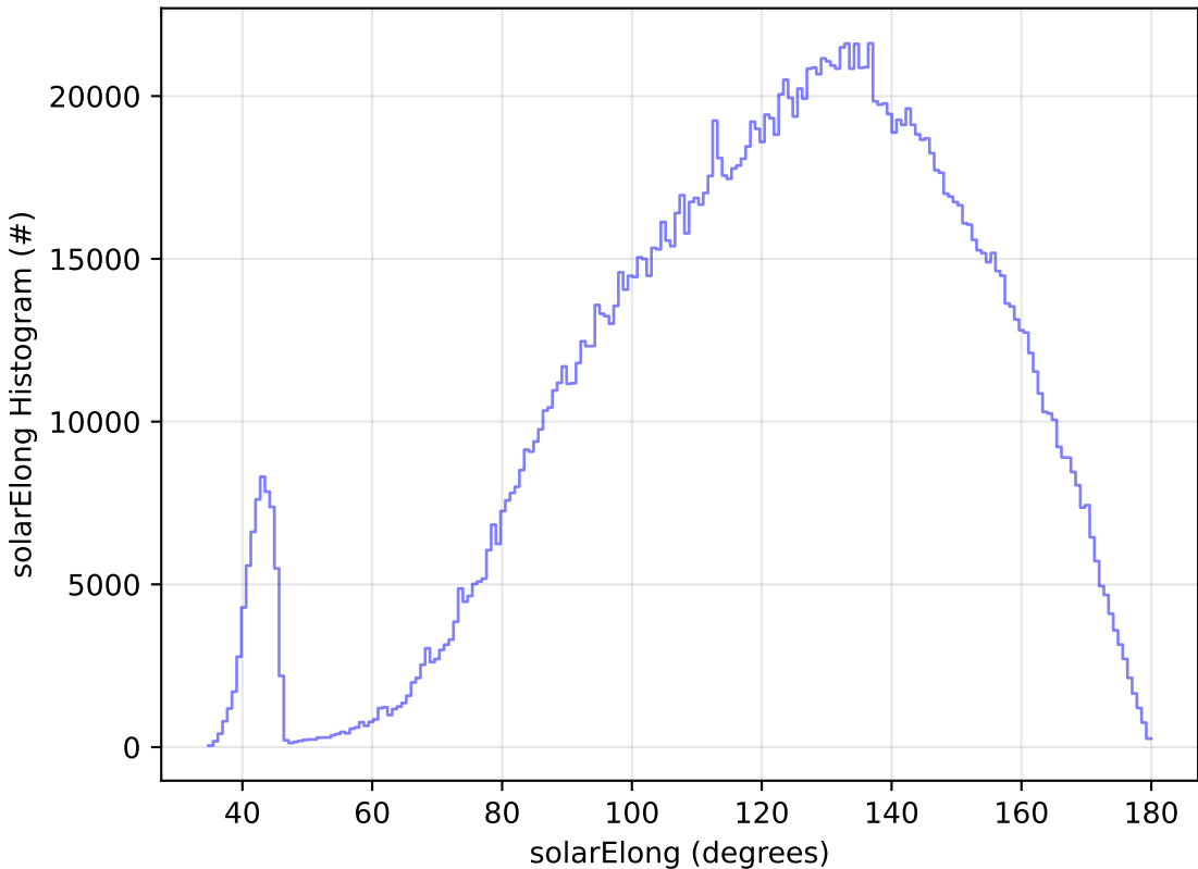
start_date_do-180v3.4_10yrs WFD all bands: solarElong Histogram
