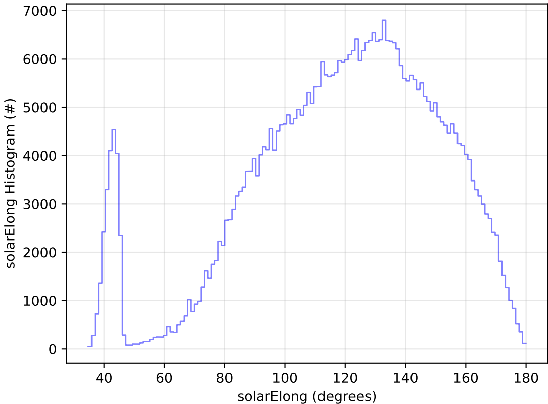
start_date_do-180v3.4_10yrs All sky z band: solarElong Histogram
