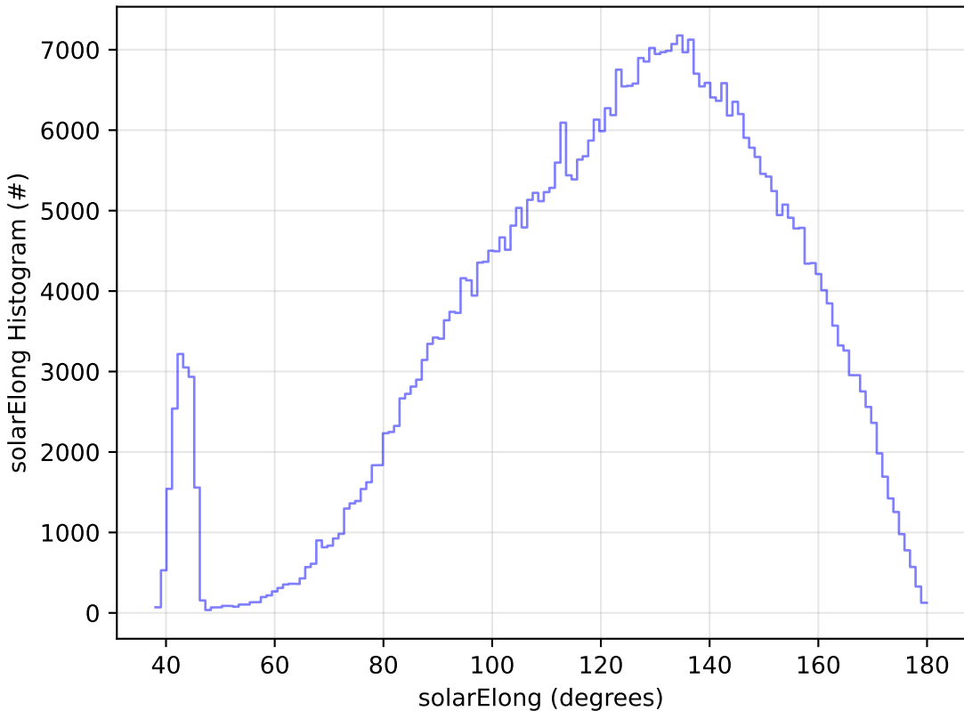
start_date_do-180v3.4_10yrs All sky r band: solarElong Histogram
